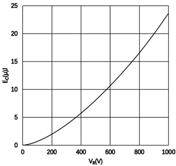
Figure 5 Typical Capacitance Energy VS Backward Voltage
