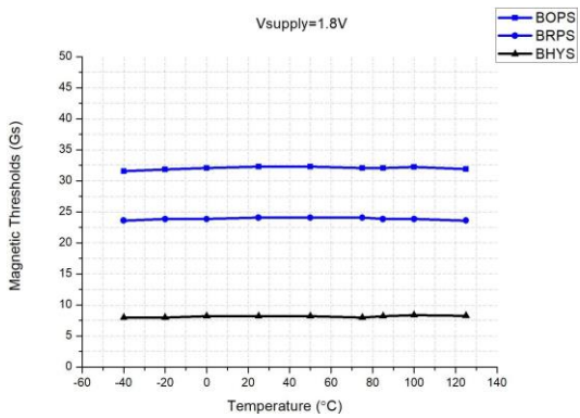
Magnetic threshold value vs temperature @ VDD=1.8\text{V}
