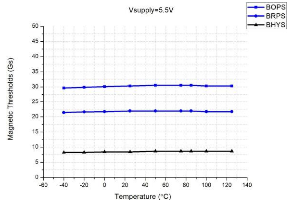
Magnetic threshold value vs temperature @ VDD=5.5\text{V}
