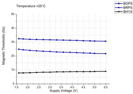
Magnetic threshold value vs. supply voltage @ T_A=25^\circ\text{C}
