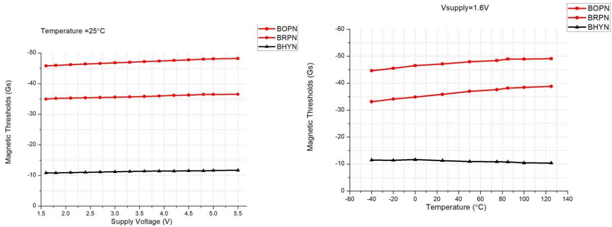
Magnetic threshold value vs. supply voltage @T A =25°C Magnetic threshold value vs temperature @VDD=1.6
