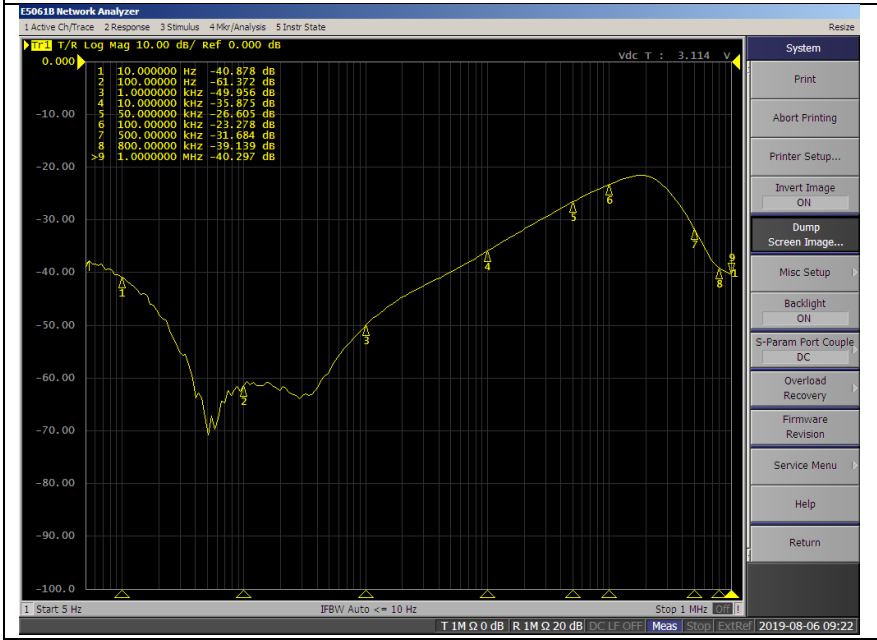
PSRR @ Iout=300mA
